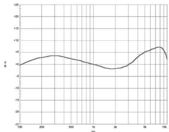
Microphone frequency response (near field) measured with B&K 4227 artificial mouth (94 dB SPL, distance of 6 mm/0.24")
